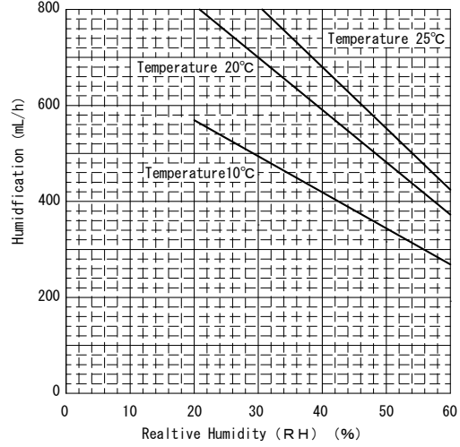
Operating Condition
